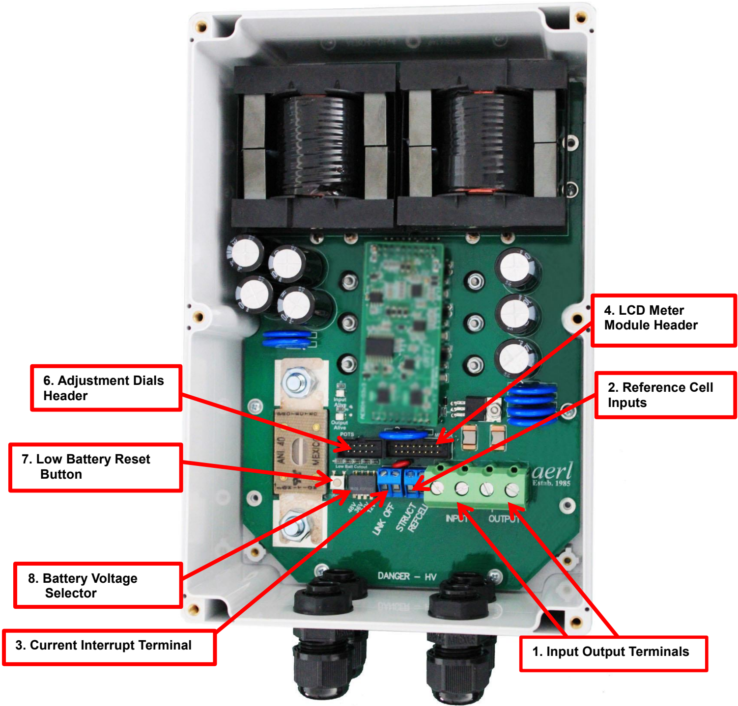
Figure 2 – PCB Layout
