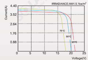
SLP060-12U I-V Curves
