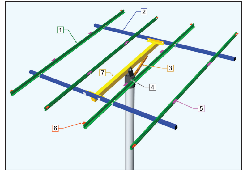
Main Structural Component
