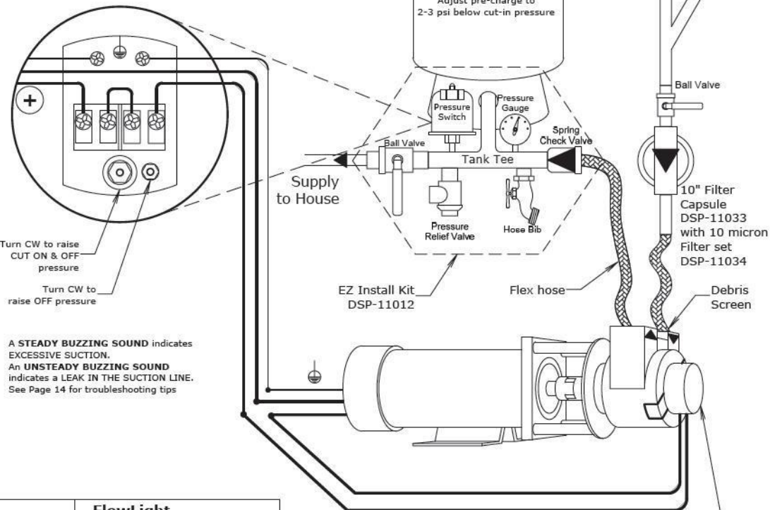
FlowLight Booster Pump EZ Install Diagram
